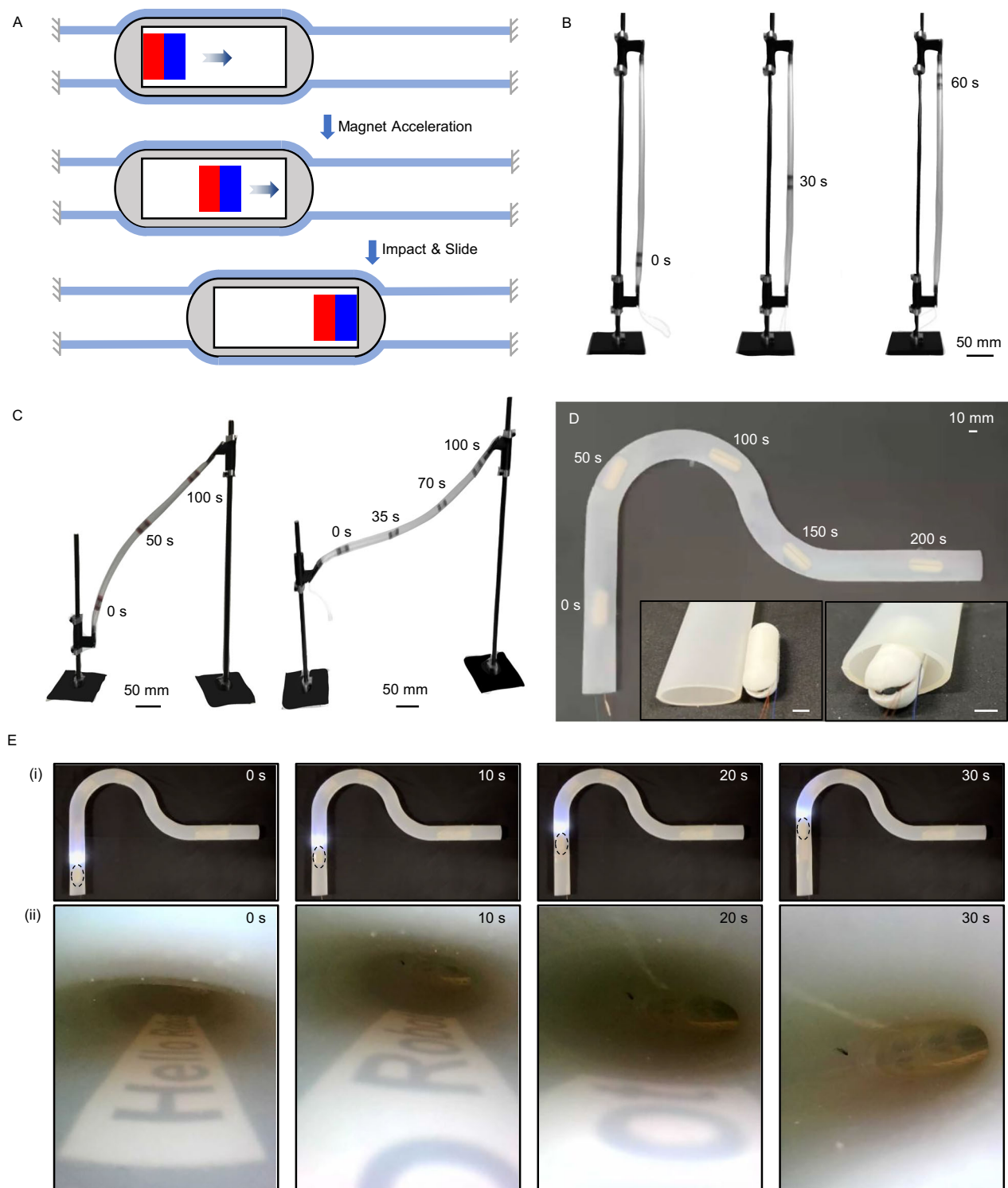
Fig. 6 | Inspection in a confined flexible tubular environment. A Schematic of MiaBot navigating a narrow, flexible silicone tube. B Locomotion in a vertical tube. C Locomotion through a tube in 3-D space. D Snapshots of MiaBot traversing straight and curved trajectories with an onboard camera. Inset: Diameter
