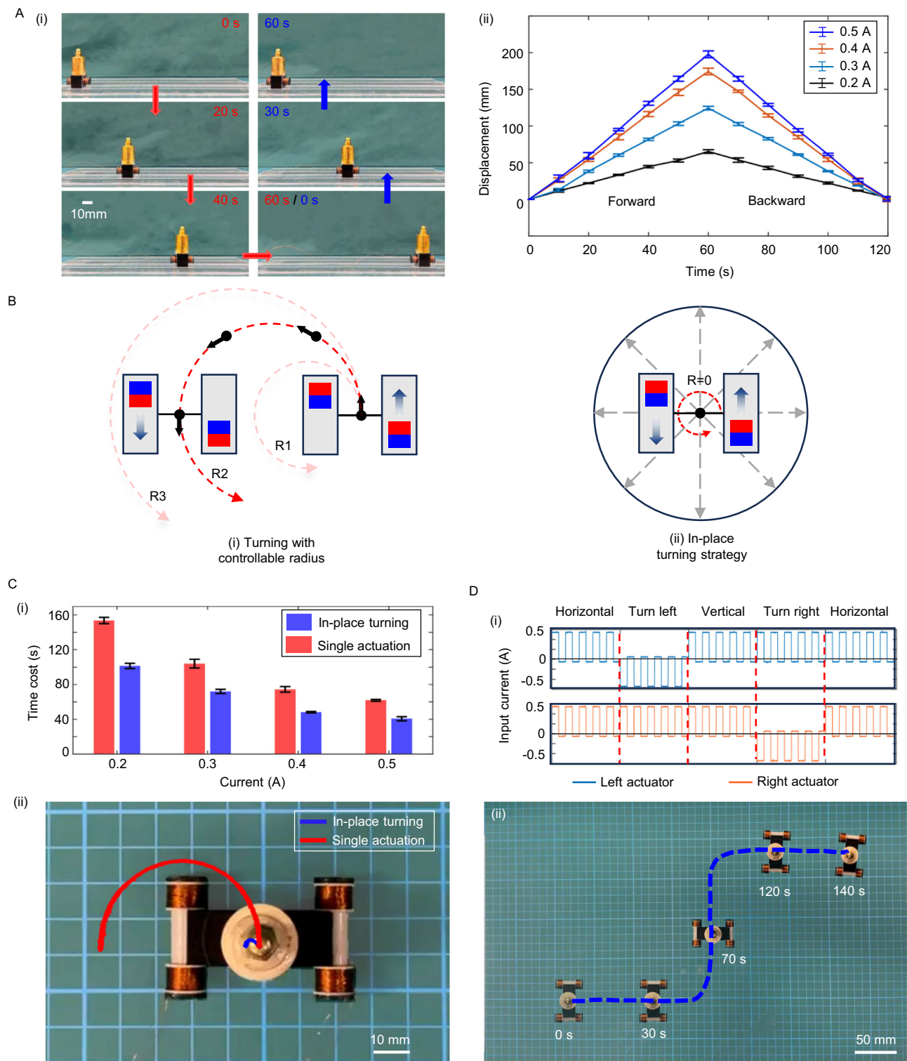
Fig. 4 | Steerability of MiaBot. A Bidirectional control: (i) Snapshots showing the MiaBot return to its initial position after 60 seconds of forward followed by 60 seconds of backward locomotion; (ii) Displacement during 120 s of forward and backward movement. B Comparison of turning strategies: (i) Conventional turning with two actuators lacking bidirectional control; (ii) Proposed in-place turning using the synergistic operation of two actuators in opposite directions.
