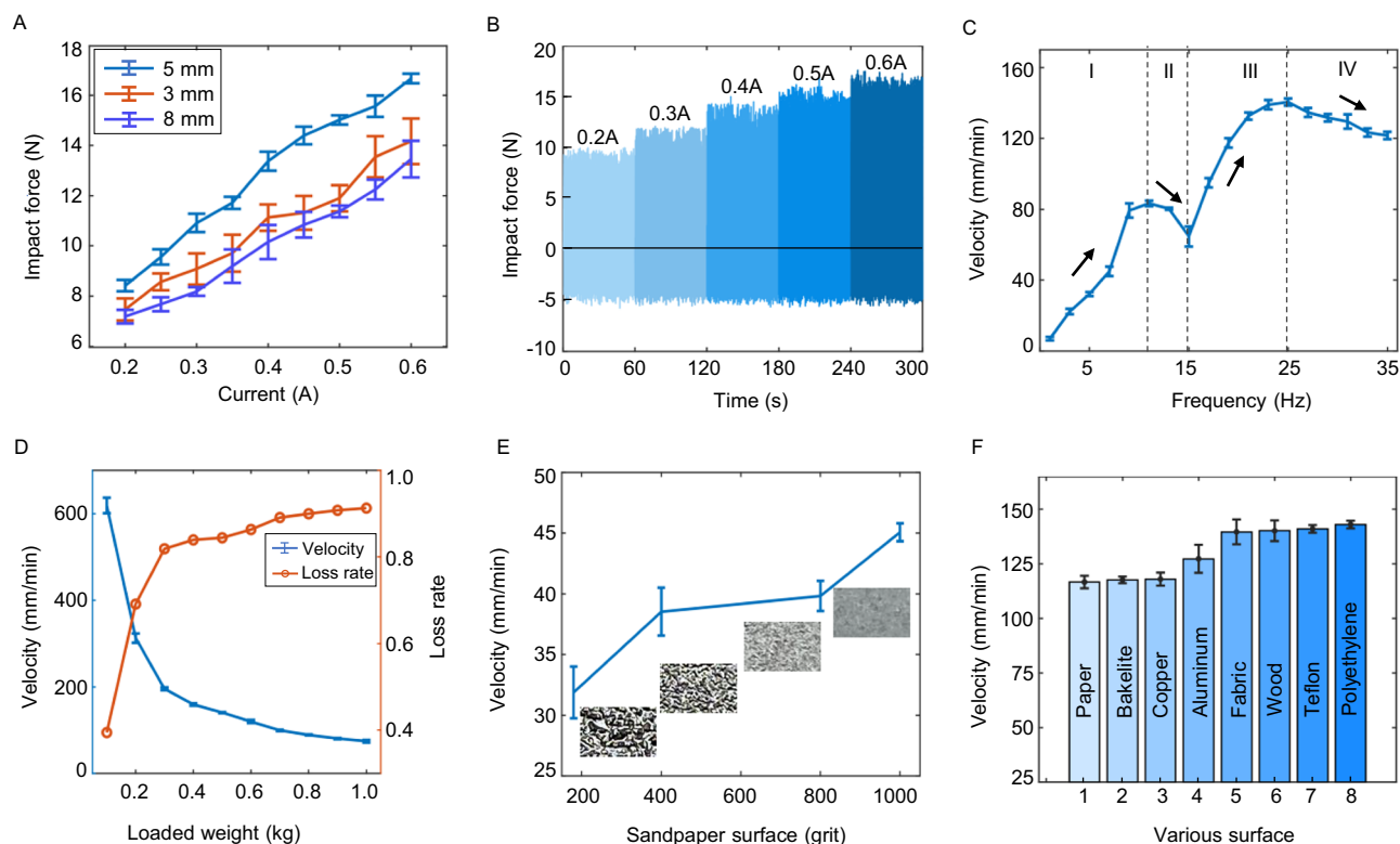
Fig. 3 | Inertial impact force and loading performance of MiaBot. A Relationship between impact force and applied current for different widths of coil set (3 mm, 5 mm, and 8 mm). B Repeatability of impact force under various actuation currents. C Locomotion velocity versus excitation frequency with a 500 g load. D The locomotion velocity decreases with increased payload, while the energy loss ratio rises
