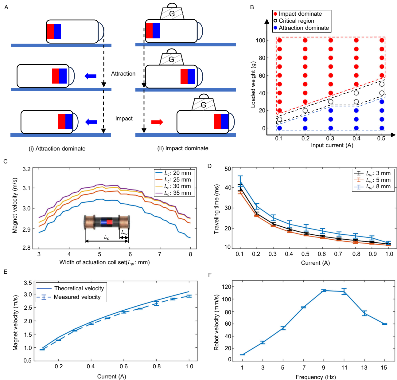
Fig. 2 | Locomotion modes and design optimization of MiaBot. A Two locomotion modes of MiaBot: (i) Without load, locomotion is dominated by the attraction force between the magnet and coils, moving the robot opposite to the magnet. (ii) With a heavy load, locomotion is dominated by the inertial impact force between the magnet and the stopper, causing the robot to move in the same direction as the magnet. B Experimental analysis of the relationship between locomotion modes and load weight under various input currents. C Numerical
