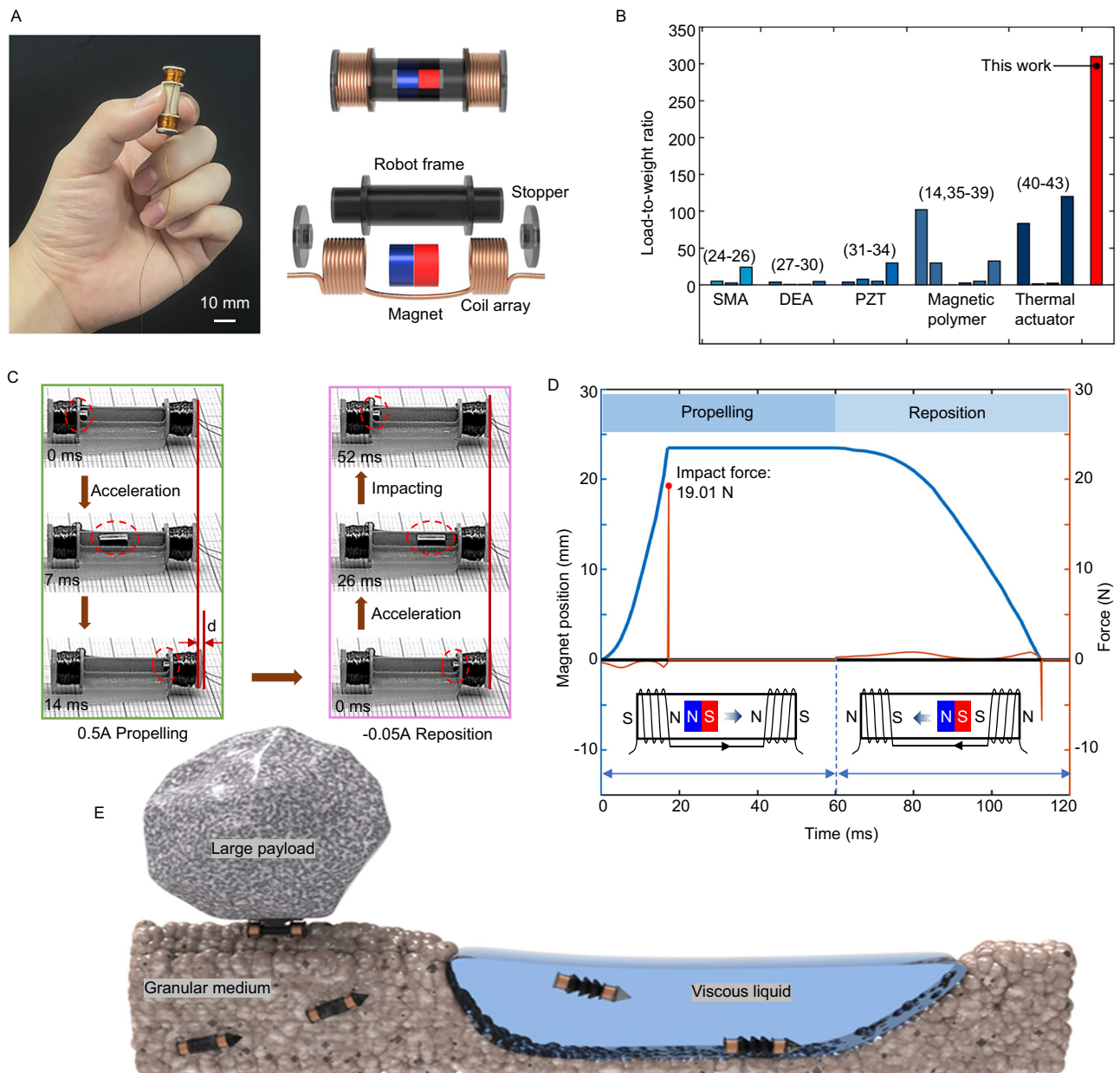
Fig. 1 | Overview and locomotion mechanism of MiaBot. A An image of a MiaBot and an exploded view of the design. B Comparison of load-carrying capability between the proposed MiaBot and the existing millirobots less than 10 g. (SMA: Shape memory alloy, DEA: Dielectric elastomer actuators, PZT: Piezoelectric actuators). C The snapshot of one actuation cycle: MiaBot carrying 500 g load actuated by a biased square wave (0.5 A and -0.05 A) signal. D Position of the inner magnet and the corresponding force on the MiaBot during one actuation cycle.
