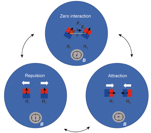
Fig. 2. The interaction between two magnetic devices. By adjusting the direction of the external magnetic field, the interaction of two magnetic substances can be converted from repulsion to attraction. \theta : the angle between the global magnetic field direction and the connecting line ( R_1 – R_2 ) of two controlled devices; \mathbf{F}_r , \mathbf{F}_\theta : the forces along and perpendicular to the connecting line, respectively.
